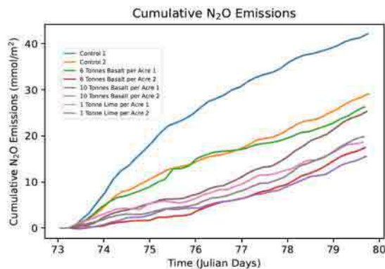
Figure 5. Example of N 2 O flux measurements in corn trials using the Picarro CRDS.
