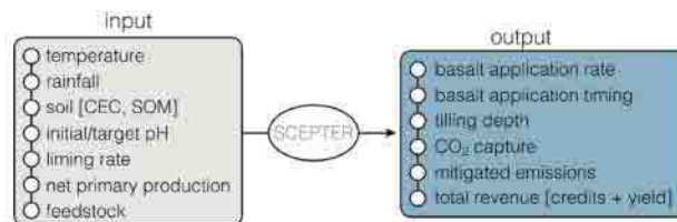
Figure 2. An overview of the SCEPTER biogeochemical model. The model takes soil characteristics and climate information to produce an optimum basalt application rate for a given crop.
